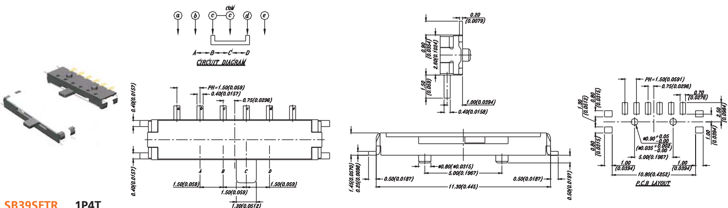
SB39SFTR 1P4T
