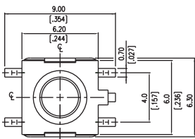
TP3SG31... SMT Terminals with Ground Terminal
