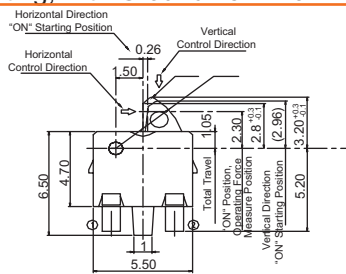
DF2RN Right Side Operating, without Ground Terminal
