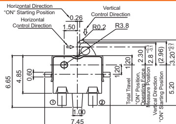
DF2RG Right Side Operating, with Ground Terminal
