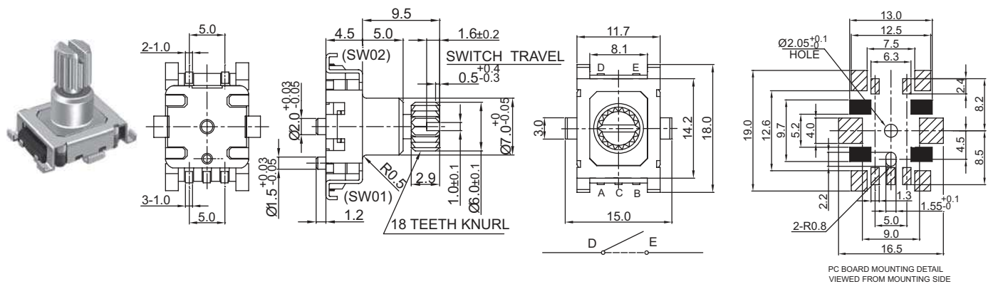
EC89SD5NBF SMT_ With Switch Travel 0.5mm, SMT Type
