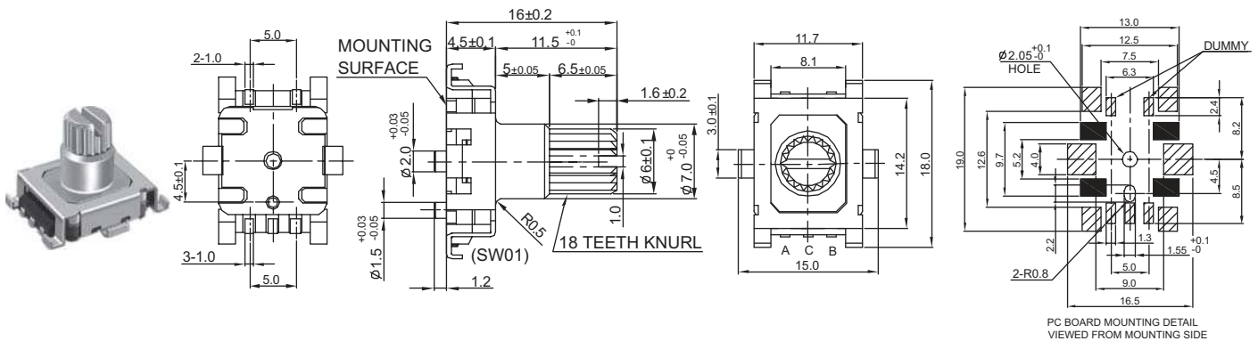
EC895NBF SMT_ Without Switch, SMT Type
