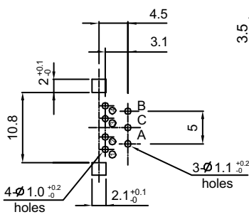
Mounting hole detail Viewed from mounting side P.C.B t=1.6mm
