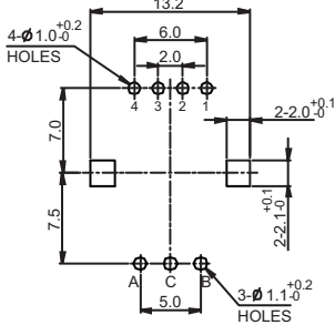
P.W.B MOUNTING DETAIL (TOLERANCE ±0.1) VIEWED FROM MOUNTING SIDE (P.C.B) t=1.5mm
